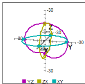
3D EIRP 1736,512 MHz
