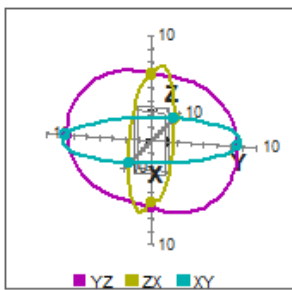
3D EIRP 868,256 MHz
