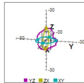
3D EIRP 2604,768 MHz
