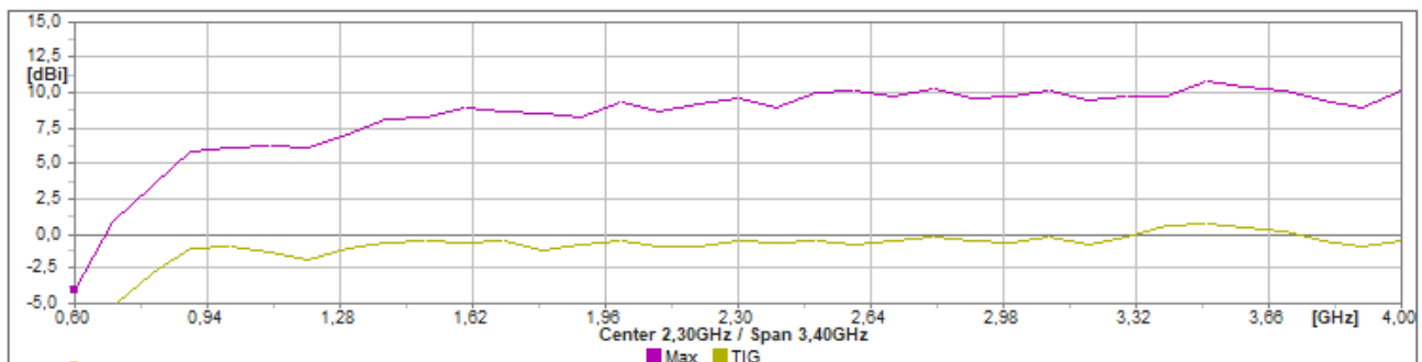
3D Gain
