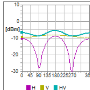
XY EIRP 915.04 MHz
