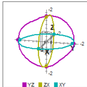
3D EIRP 915.04 MHz
